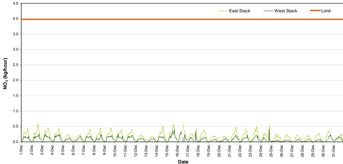
Figure 18: Nitrogen Dioxide Mass Rate (1 Hour Average)
