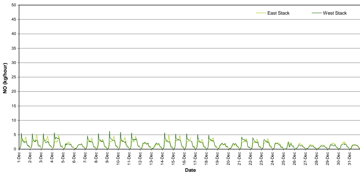
Figure 17: Nitric Oxide Mass Rate (1 Hour Average)
