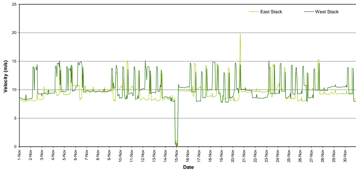
Figure 13: Stack Velocity (1 Hour Average)
