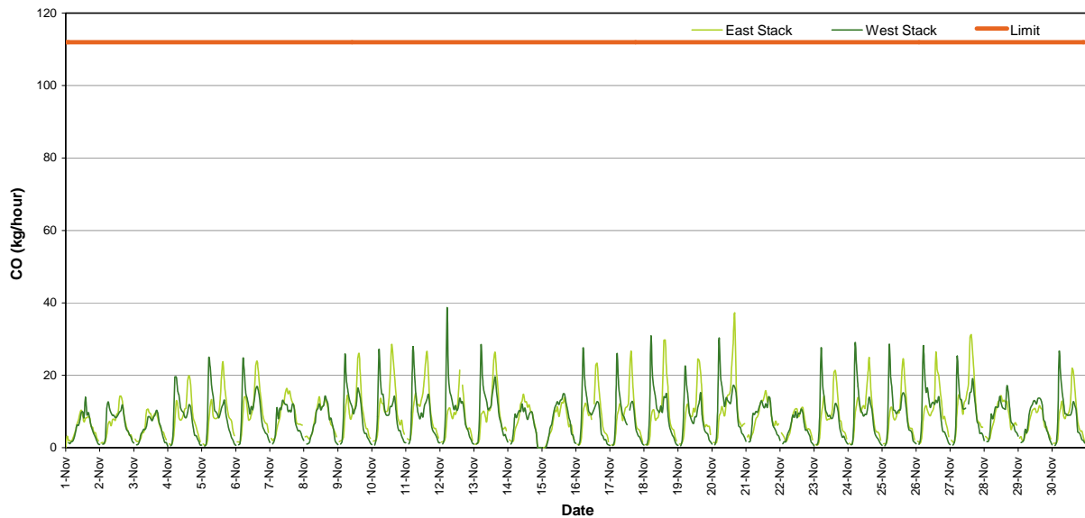
Figure 10: Carbon Monoxide Mass Rate (1 Hour Average)
