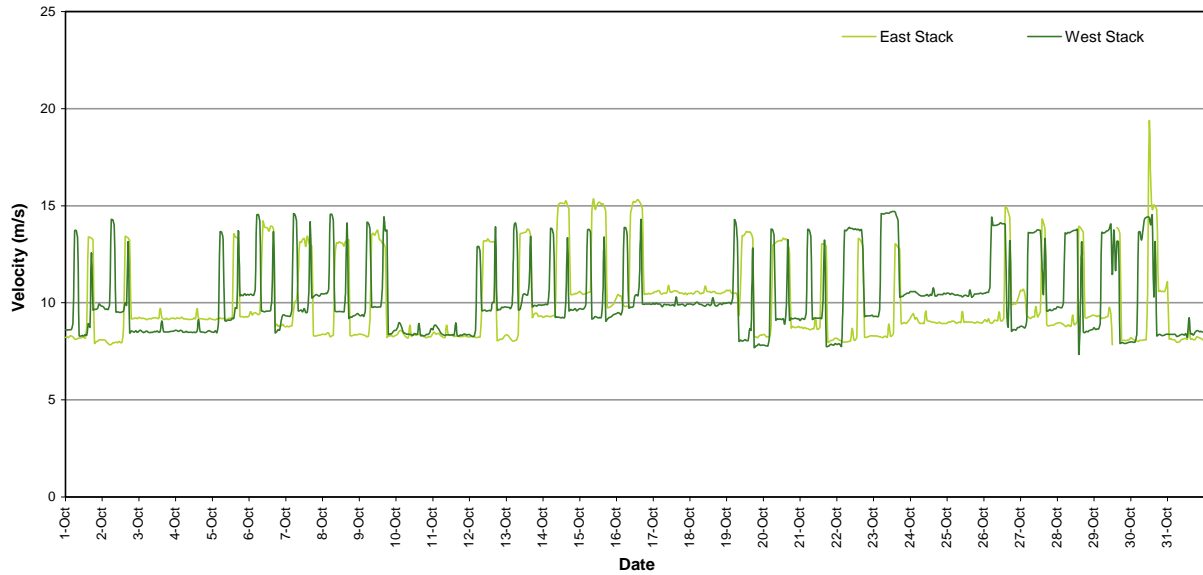
Figure 7: Stack Velocity (1 Hour Average)
