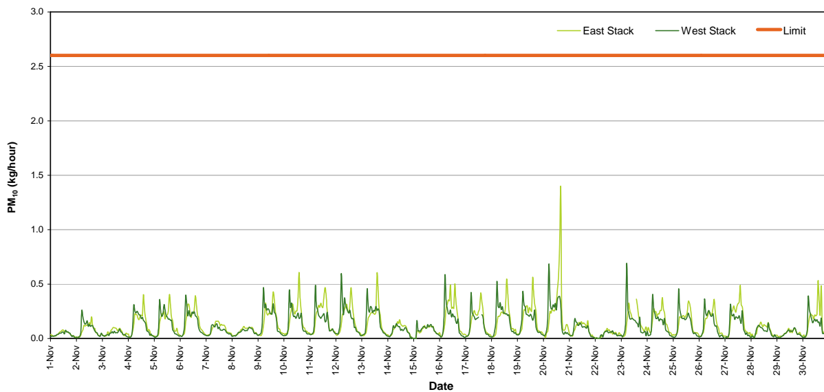
Figure 9: PM 10 Mass Rate (1 Hour Average)
