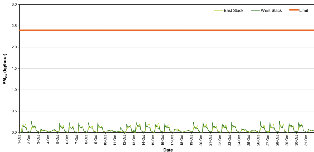
Figure 2: PM 2.5 Mass Rate (1 Hour Average)
