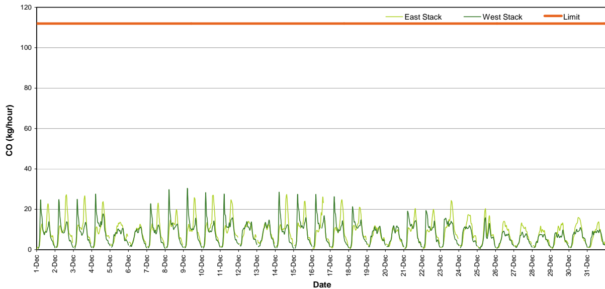
Figure 16: Carbon Monoxide Mass Rate (1 Hour Average)
