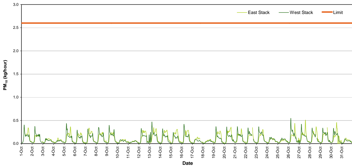
Figure 3: PM 10 Mass Rate (1 Hour Average)
