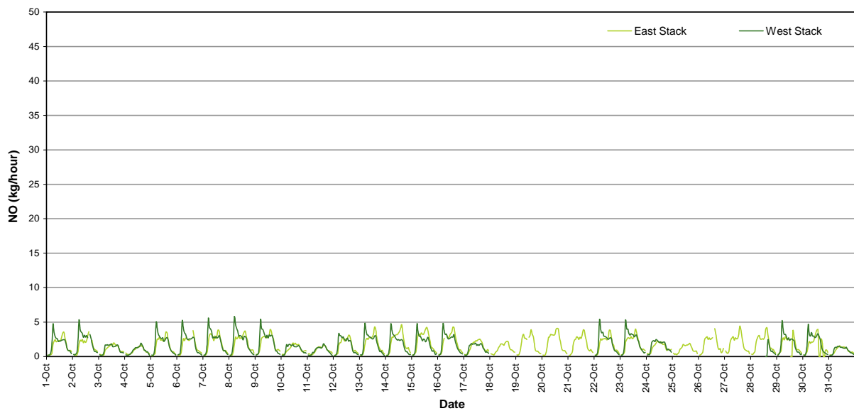
Figure 5: Nitric Oxide Mass Rate (1 Hour Average)
