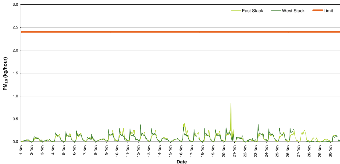
Figure 8: PM 2.5 Mass Rate (1 Hour Average)
