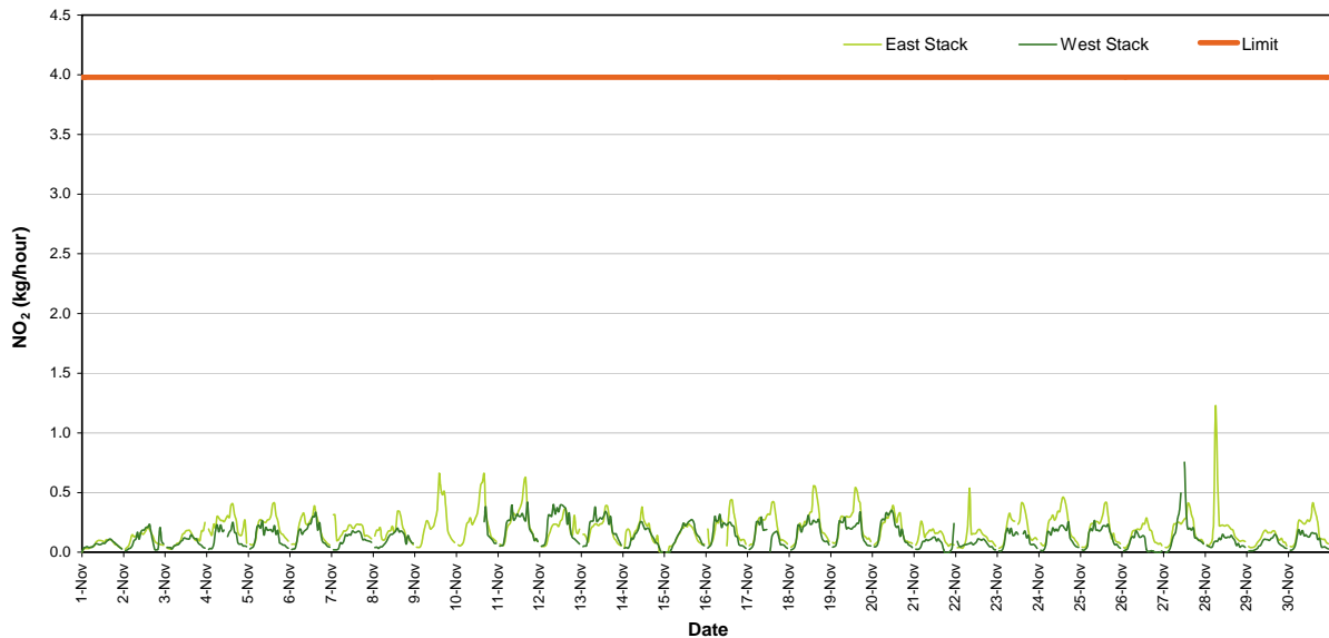
Figure 12: Nitrogen Dioxide Mass Rate (1 Hour Average)
