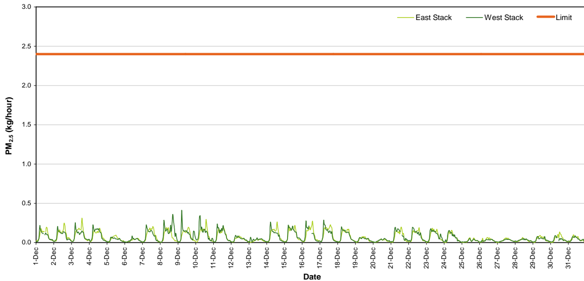
Figure 14: PM 2.5 Mass Rate (1 Hour Average)
