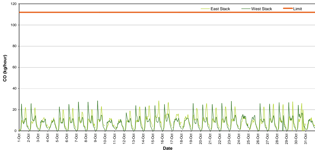
Figure 4: Carbon Monoxide Mass Rate (1 Hour Average)
