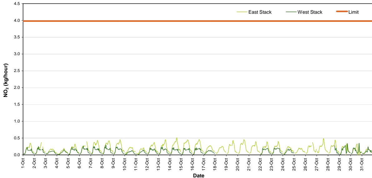
Figure 6: Nitrogen Dioxide Mass Rate (1 Hour Average)
