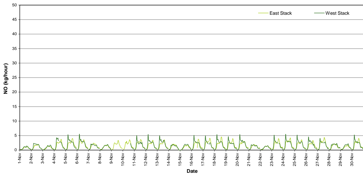
Figure 11: Nitric Oxide Mass Rate (1 Hour Average)
