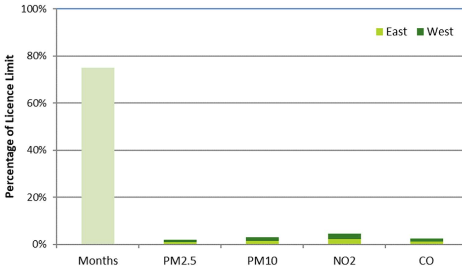
Figure 20: Ventilation Stack Emissions as Percentage of Licence Limit (1/07/2018 – 31/03/2019)
