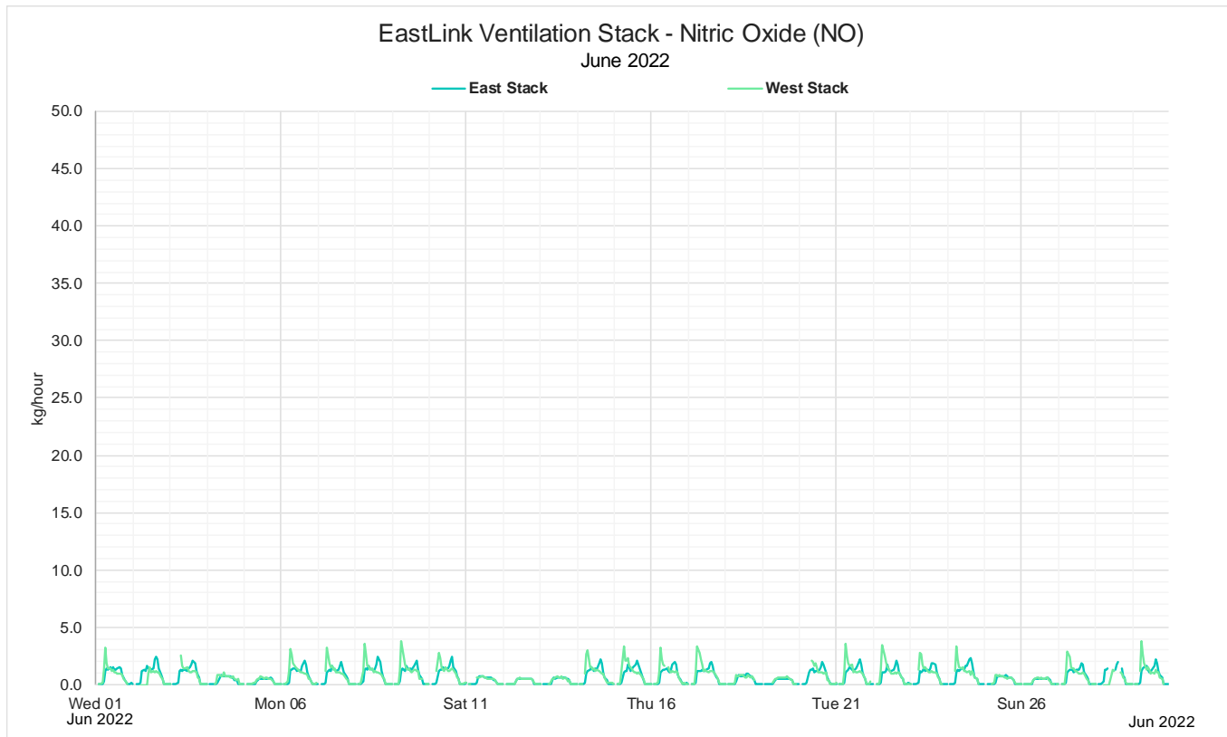
Figure 15: June 2022 Monthly 1 hour mass rate NO
