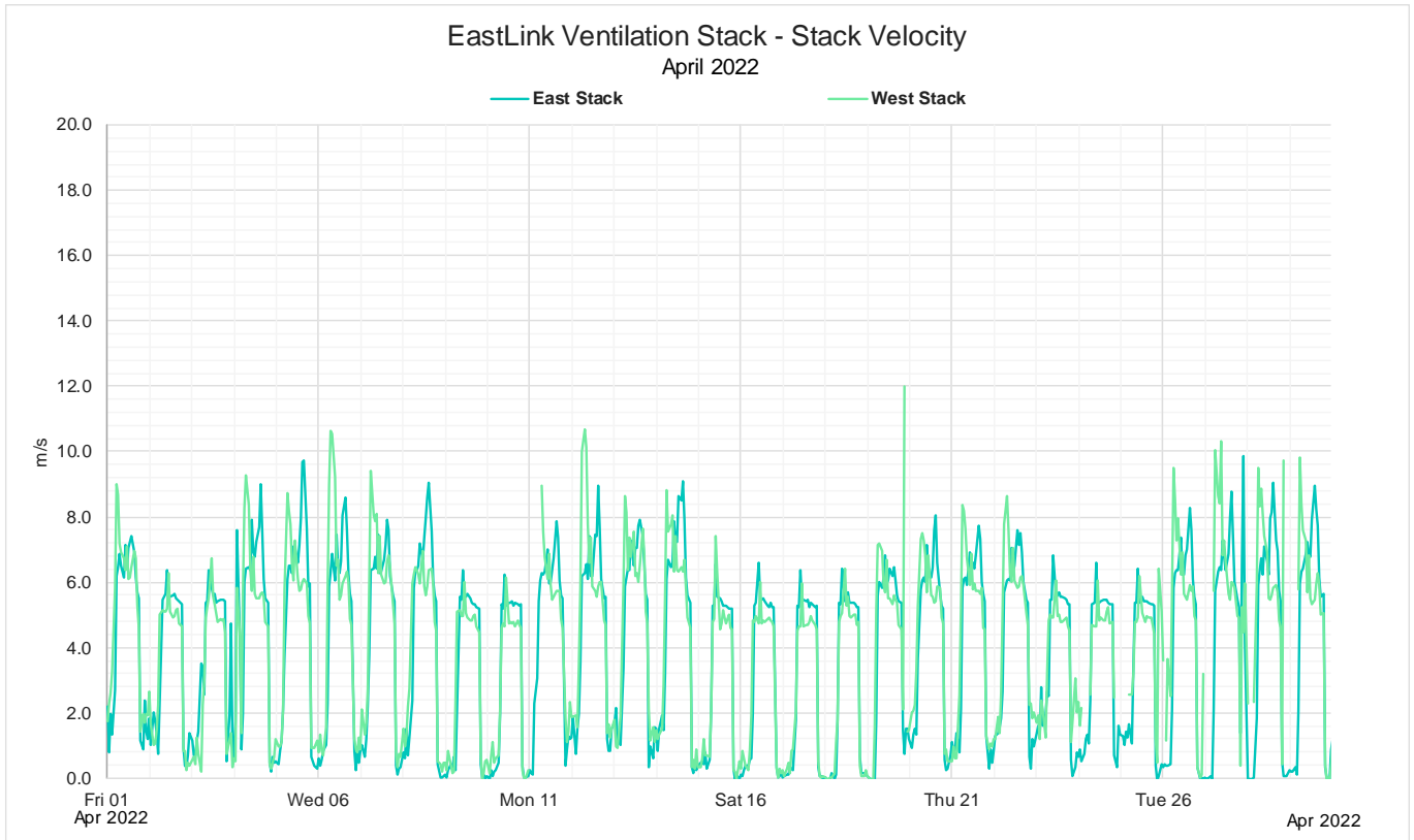
Figure 7: April 2022 Monthly 1 hour average stack velocity
