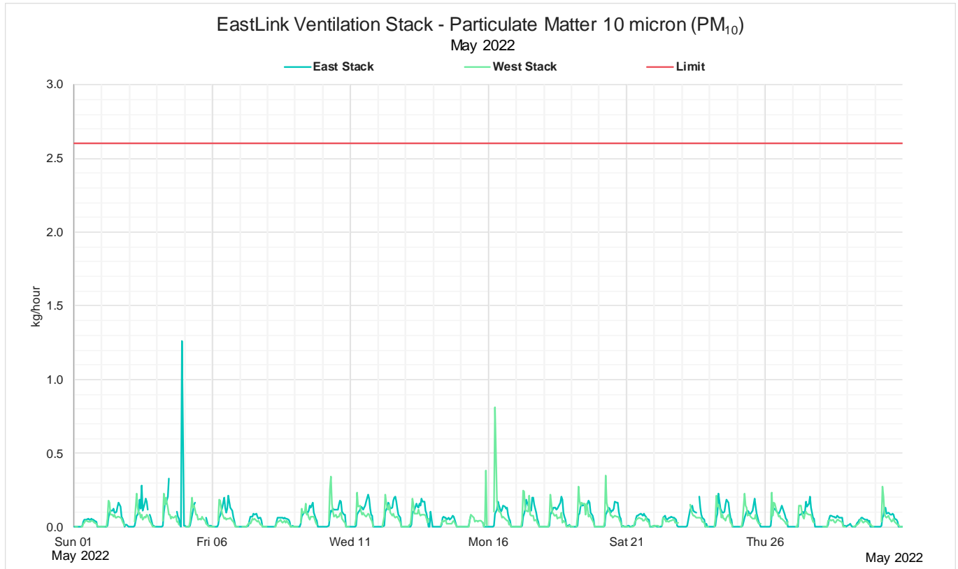
Figure 12: May 2022 Monthly 1 hour mass rate PM 10
