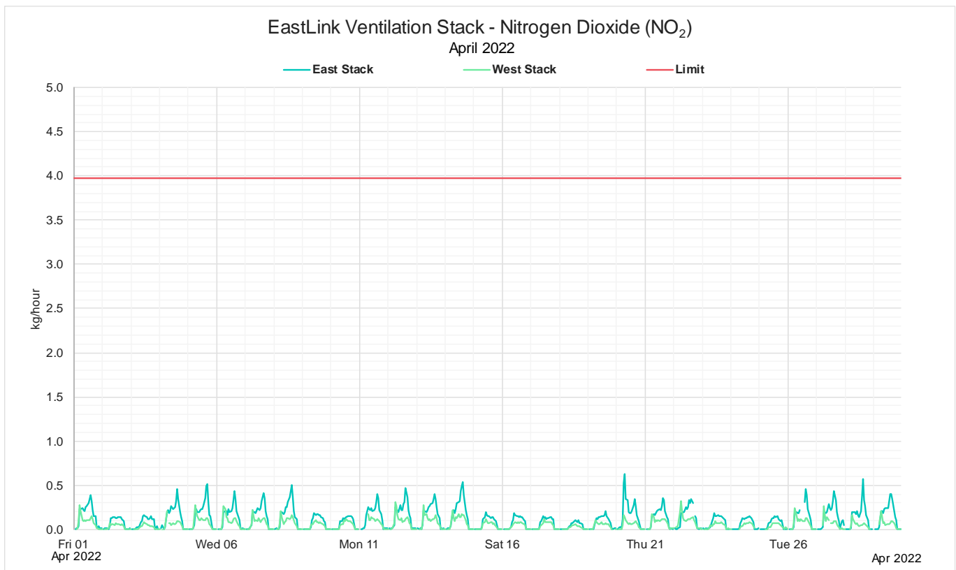
Figure 2: April 2022 Monthly 1 hour mass rate NO 2
