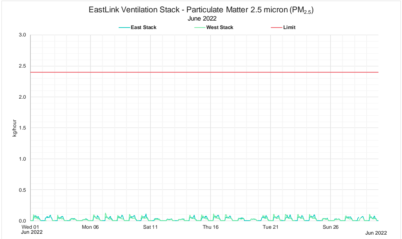
Figure 17: June 2022 Monthly 1 hour mass rate PM 2.5
