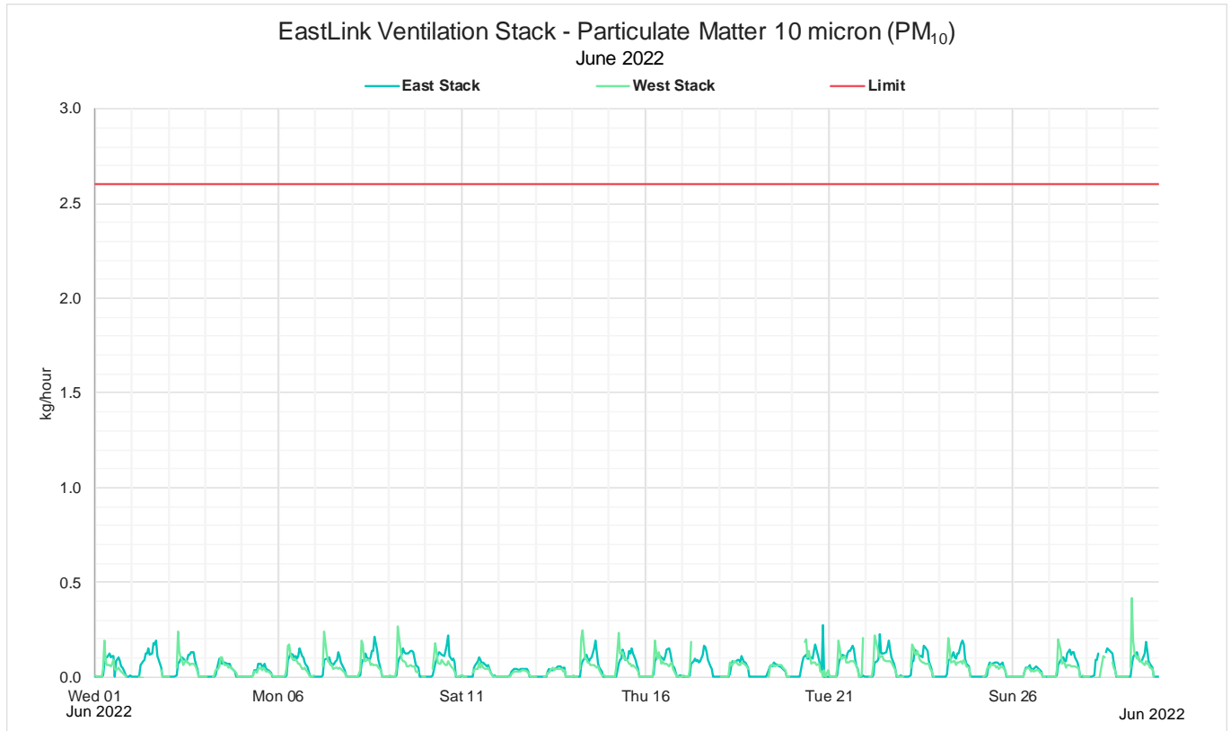
Figure 18: June 2022 Monthly 1 hour mass rate PM 10
