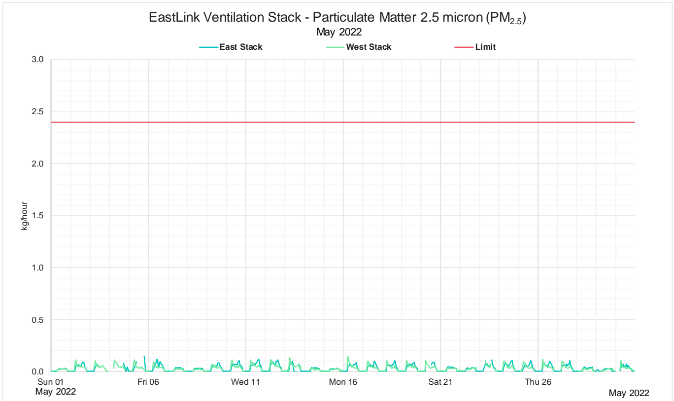
Figure 11: May 2022 Monthly 1 hour mass rate PM 2.5
