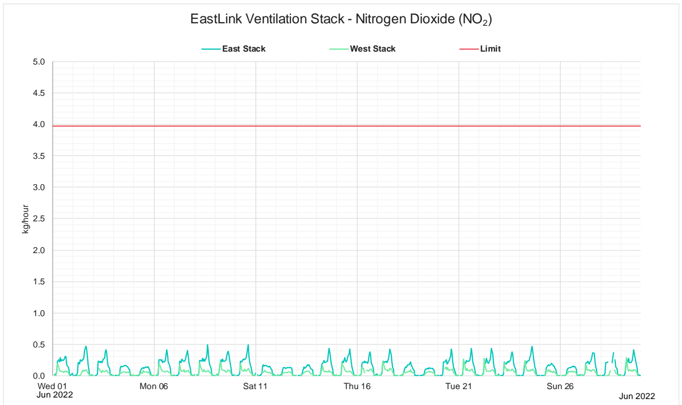
Figure 14: June 2022 Monthly 1 hour mass rate NO 2
