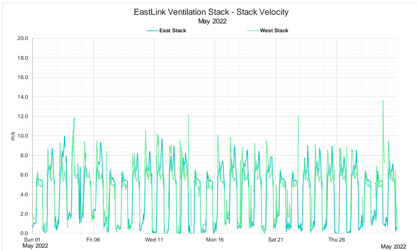
Figure 13: May 2022 Monthly 1 hour average stack velocity
