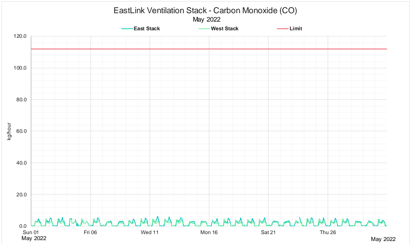
Figure 10: May 2022 Monthly 1 hour mass rate CO
