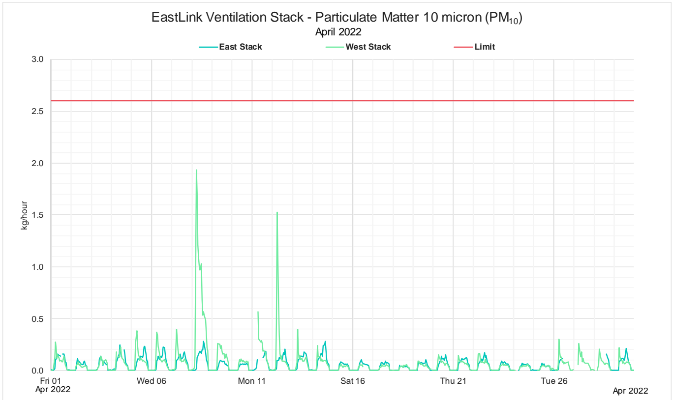
Figure 6: April 2022 Monthly 1 hour mass rate PM 10
