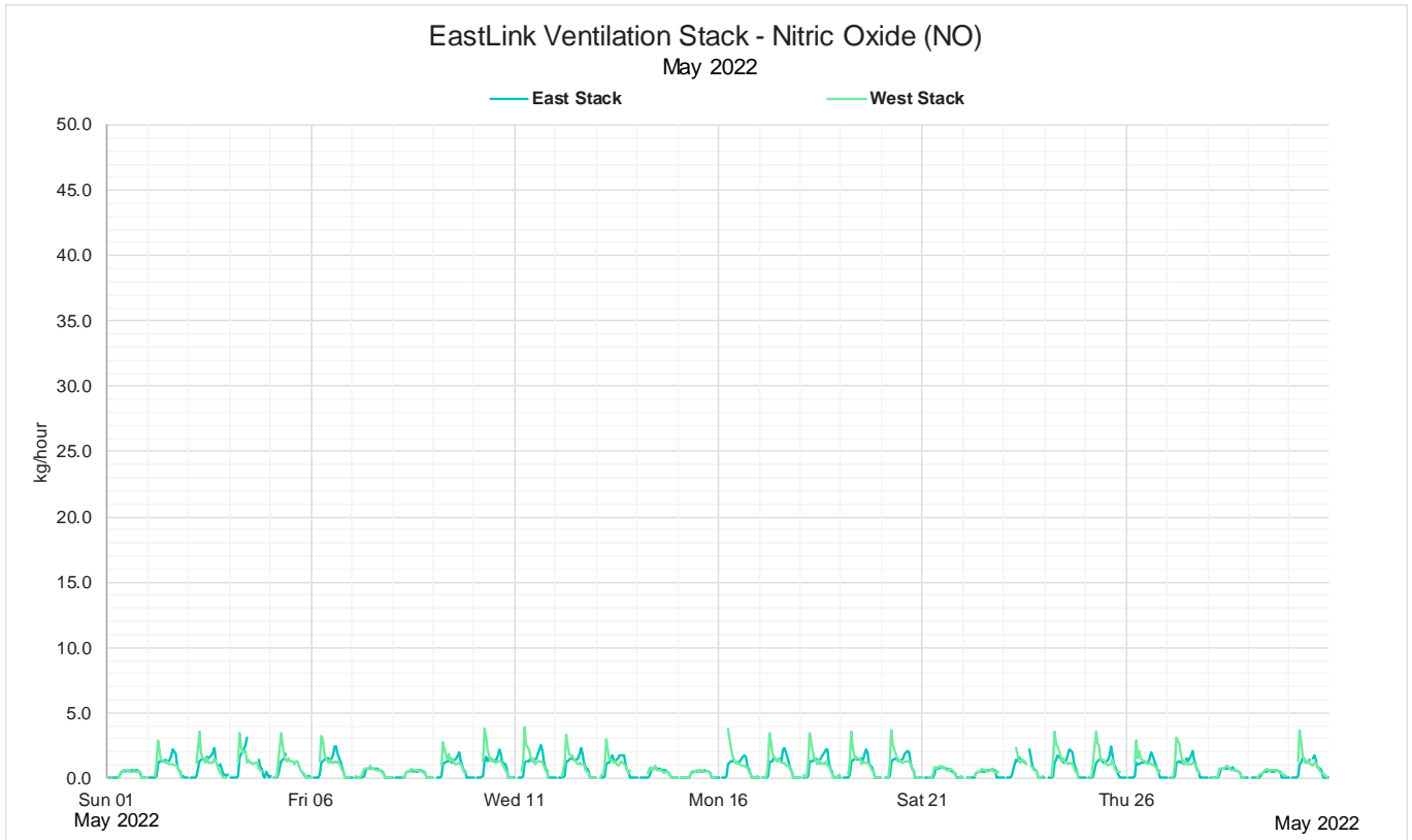
Figure 9: May 2022 Monthly 1 hour mass rate NO
