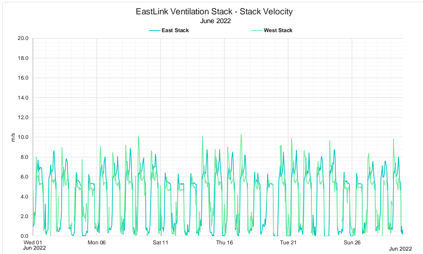
Figure 19: June 2022 Monthly 1 hour average stack velocity
