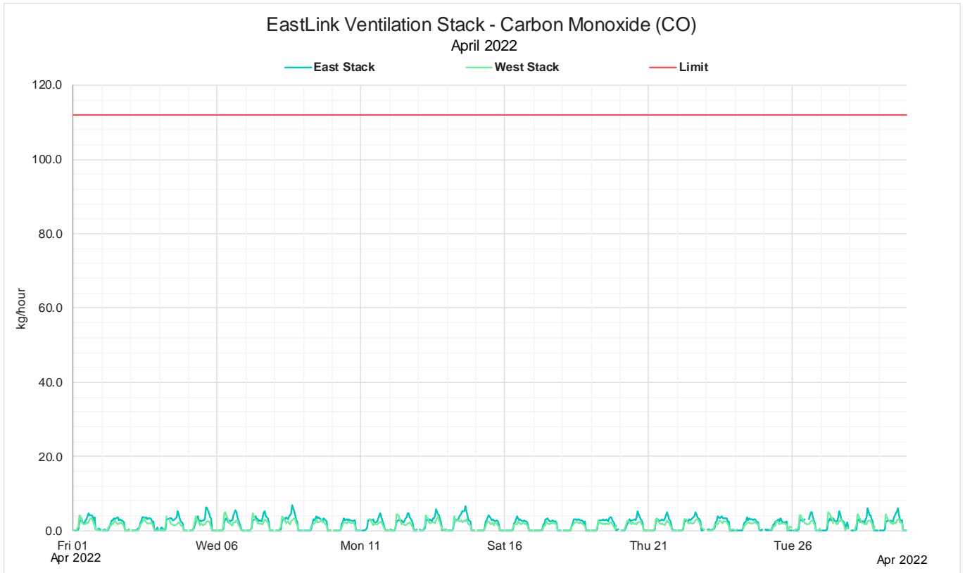
Figure 4: April 2022 Monthly 1 hour mass rate CO
