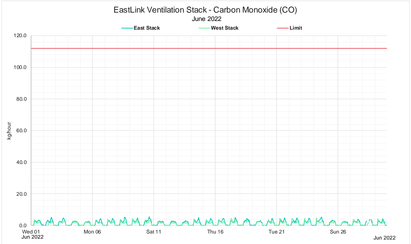
Figure 16: June 2022 Monthly 1 hour mass rate CO
